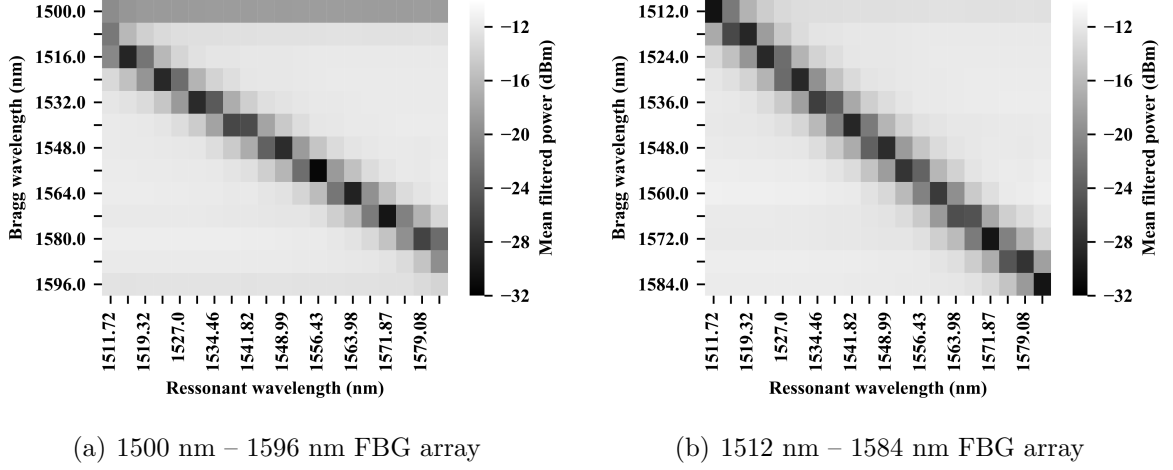
Figure 10 – Relationship between filtered power by each FBG and the LPG resonant wavelength for two FBG arrays.
