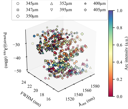
Figure 9 – Spectral features of all spectra considered for the ANN-based interrogation method.
