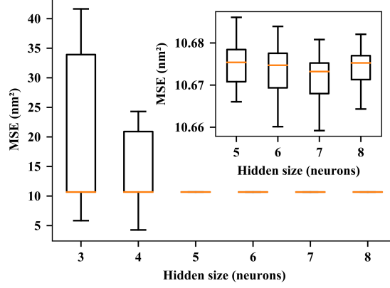
Figure 11 – Relationship between hidden layer size (number of neurons) and validation mean squared error for the 20 experiments per configuration.
