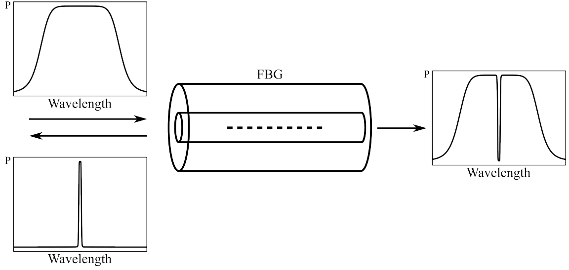
Figure 1 – Schematic of the light passing through an FBG.
