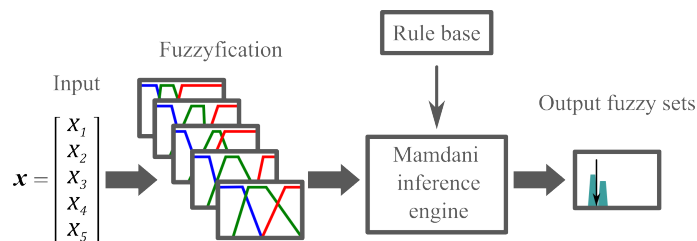
Figure 14 – Schematic of a fuzzy inference system.
