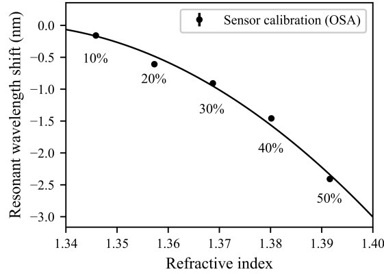
Figure 40 – LPG sensor calibration.
