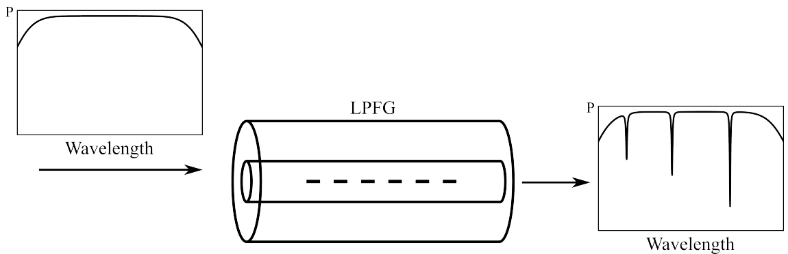
Figure 2 – Schematic of the light passing through an LPG.
