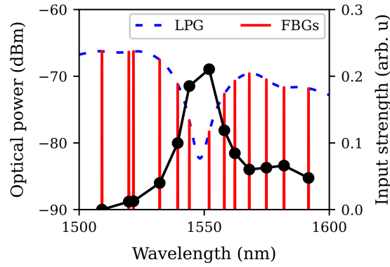
Figure 31 – Preprocessing example.
